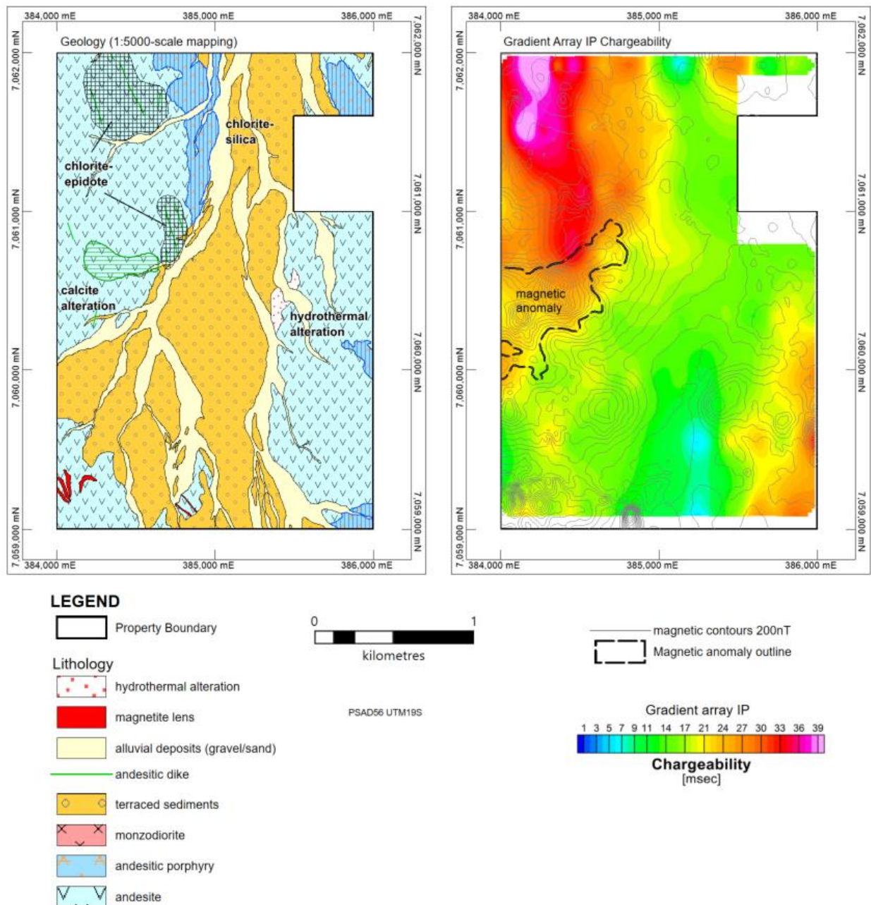
Figure 4. Summary of the geological mapping (including alteration) (left) and the gradient array IP chargeability data from the recent work program (right).
