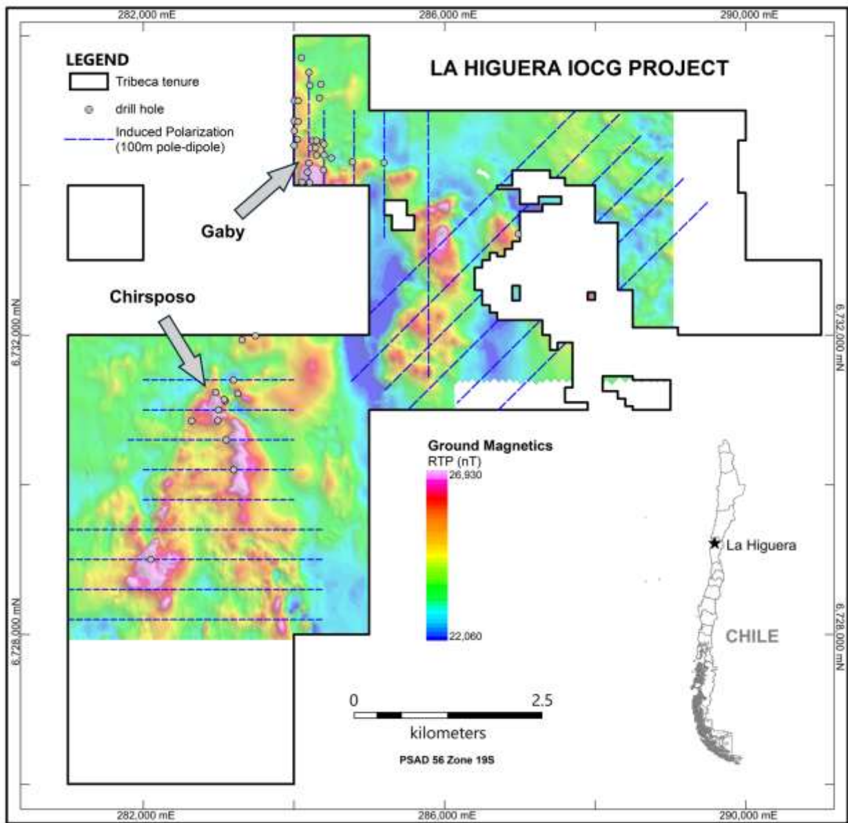
Figure 1. Location of the Gaby and Chirposo targets within the La Higuera IOCG Project outline.
