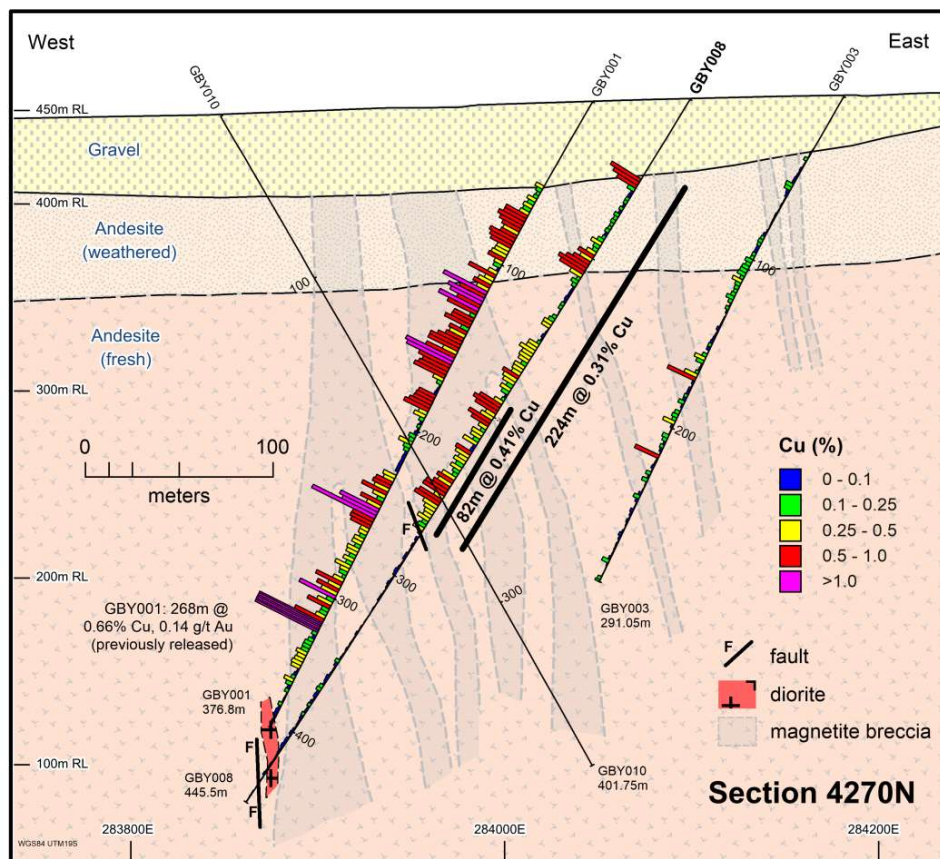
Figure 1. Cross-section 4270N with the location of GBY008 shown. Drill hole GBY010, drilled back from the west, has been completed with logging and sampling in progress. The orientation of the faults as shown is unconstrained. The histogram bars showing copper grade in GBY001 have been top-cut at 2% Cu.
